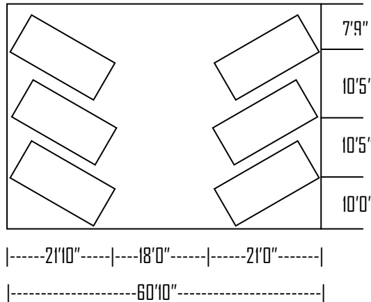
60° STANDARD PARKING
