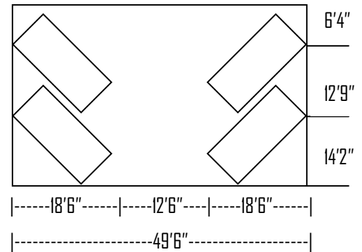
45° STANDARD PARKING
