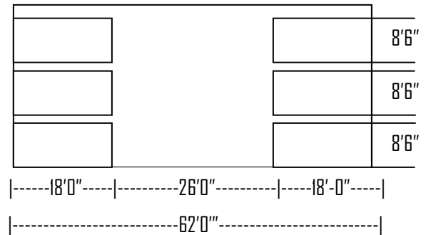
90° STANDARD PARKING
