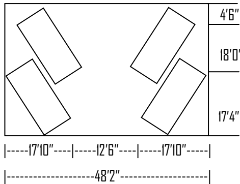
30° STANDARD PARKING
