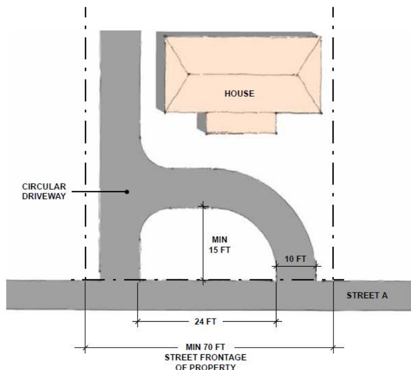
Figure 17.70-3 – Circular Driveway
