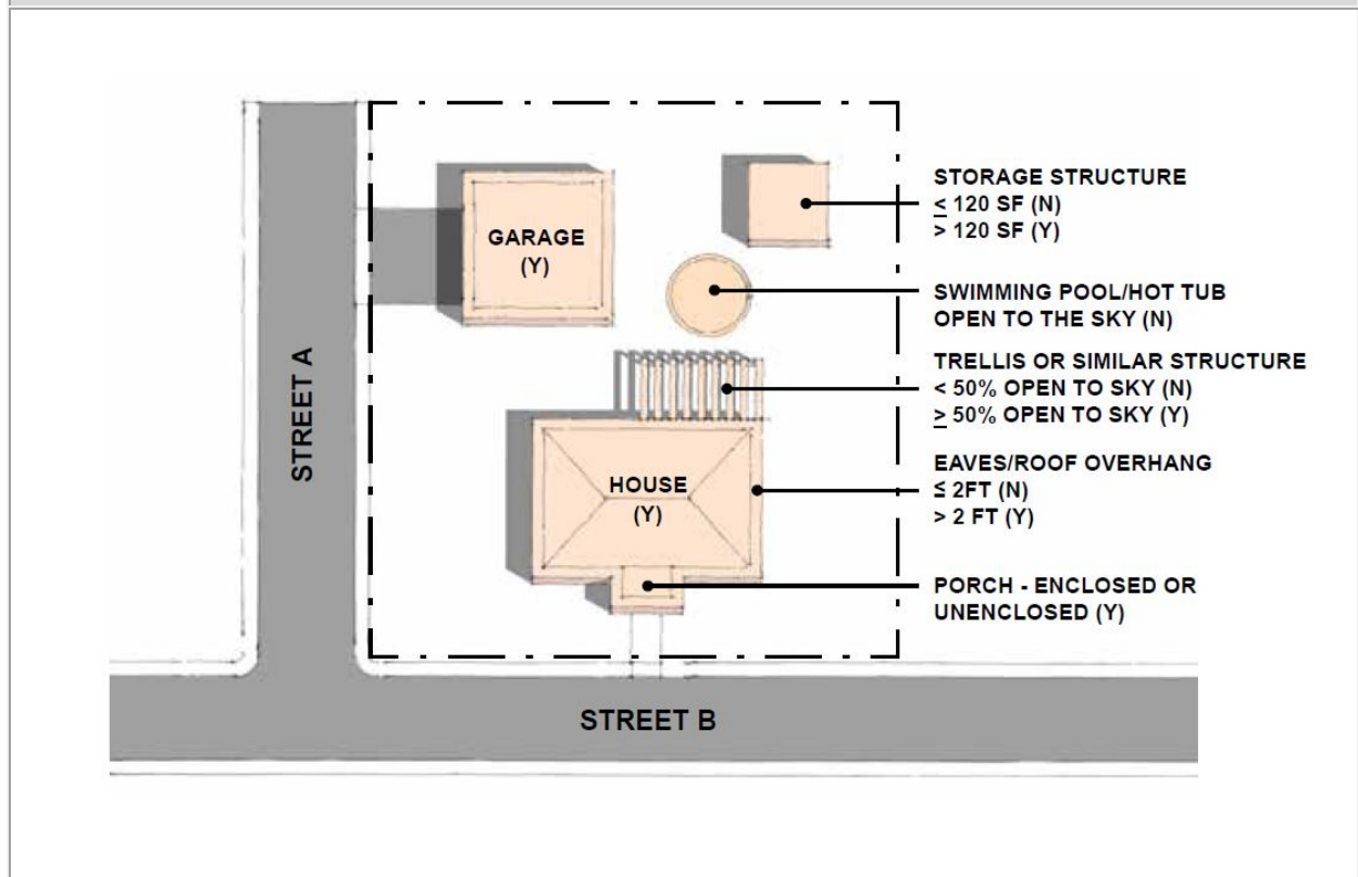
Figure 17.12-3 – Lot Coverage
